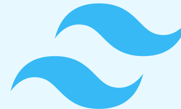
Tailwindcss
