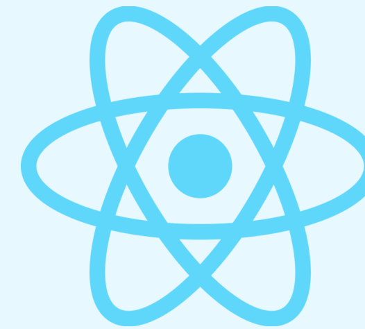
React
